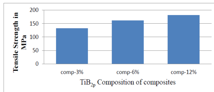
Figure 3. Tensile Strength
